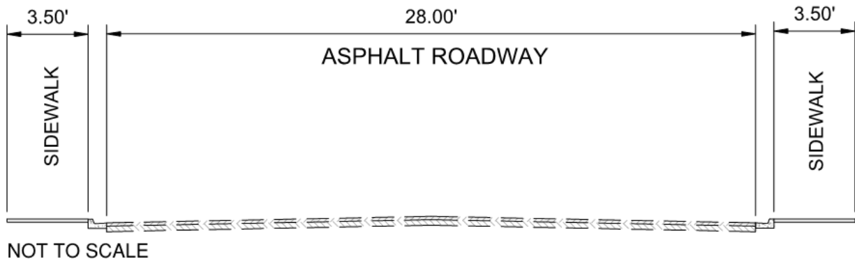
Figure 5: Arizona Street Existing Typical Section
